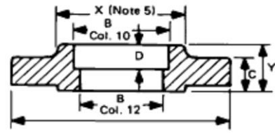
Socket Welding (1/2" to 3" only)
