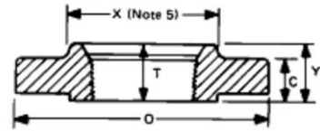
Threaded
